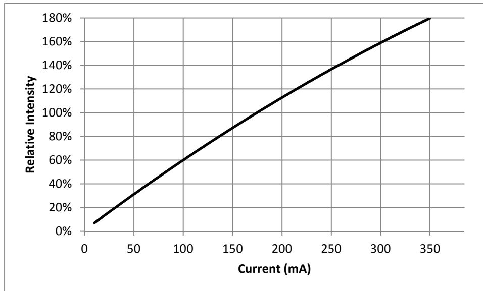
Figure 4: Typical Flux vs. Current – BXRE-xxx0400-A-xx
