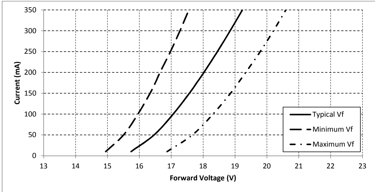
Figure 2: Typical Current vs. Voltage ( T_j=T_c=25^\circ\text{C} ) – BXRE-xxx0400-A-xx
