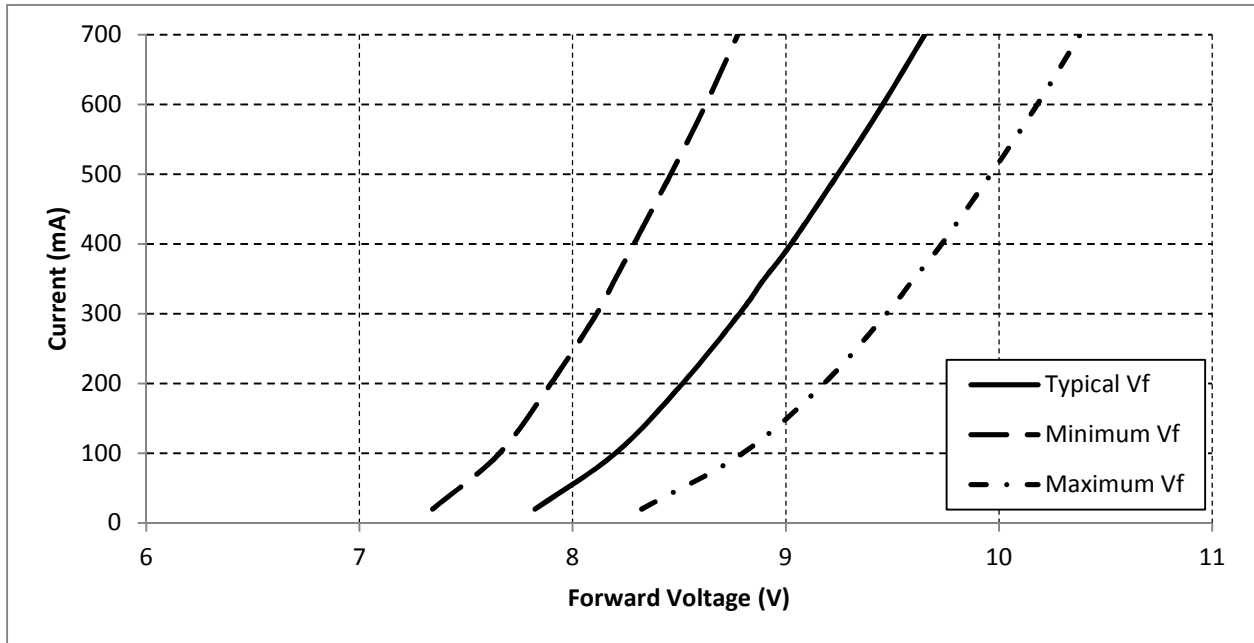
Figure 3: Typical Current vs. Voltage ( T_j=T_c=25^\circ\text{C} ) – BXRE-xxx0400-B-xx
